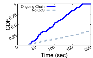
Figure 16: Ongoing Chain Prioritization completion times
