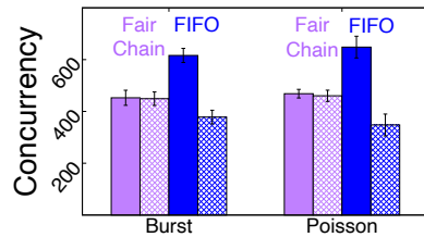
Figure 20: Fairness with realistic workloads: Compile (solid), sCV (dashed)
