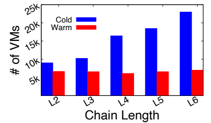
Figure 11: Resource allocation in linear chain analysis
