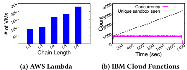
Figure 7: Inefficient resource allocation
