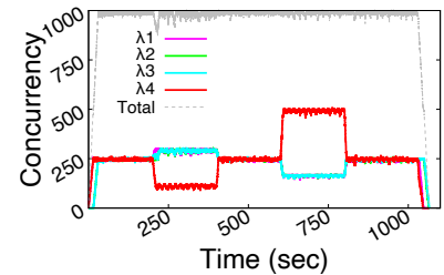
Figure 15: Reactive Concurrency Sharing with adaptive workload
